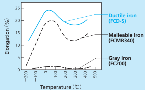
Elongation
