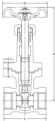
End to end : JV 4-4 End connection : JIS B 0203
