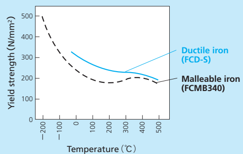
Yield strength
