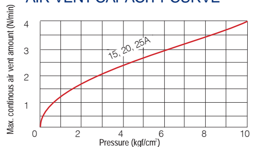
AIR-VENT CAPACITY CURVE
